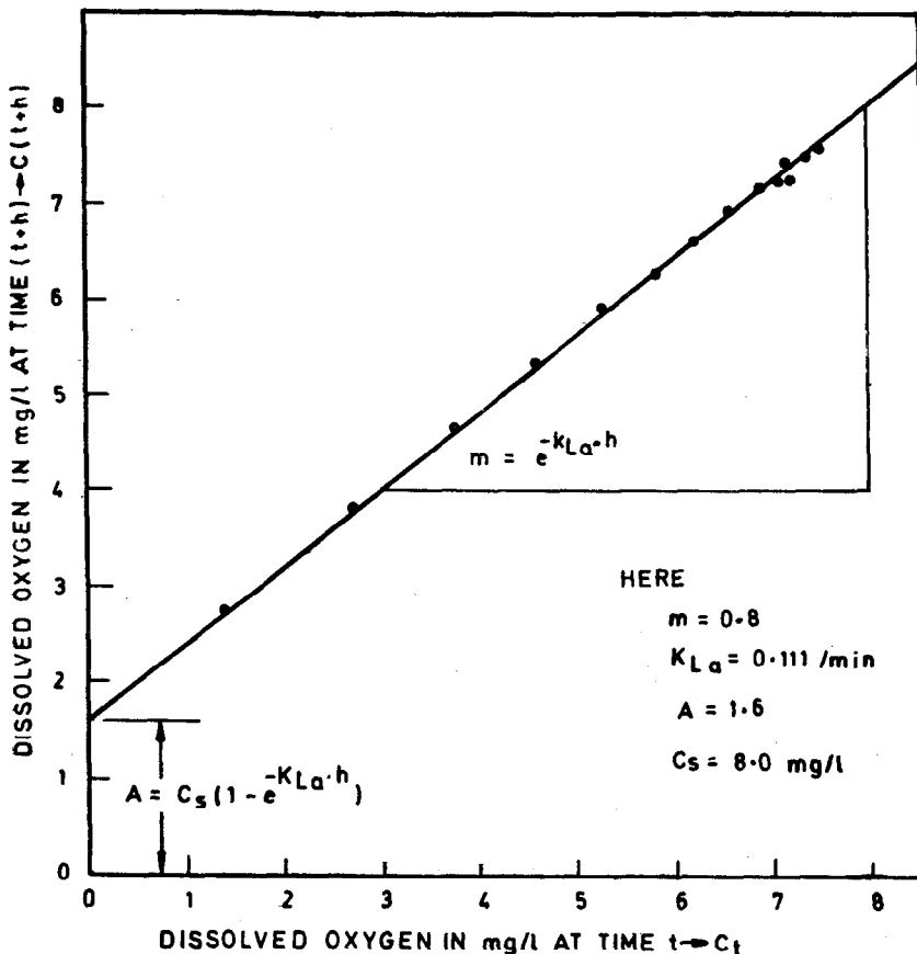
FIG. 3 METHOD OF DETERMINATION OF K_{La}
